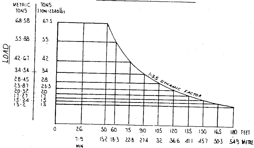
RADIUS LOAD CAPACITY CHART 180'-0" LONG JIB - 3 FALL HOOK
