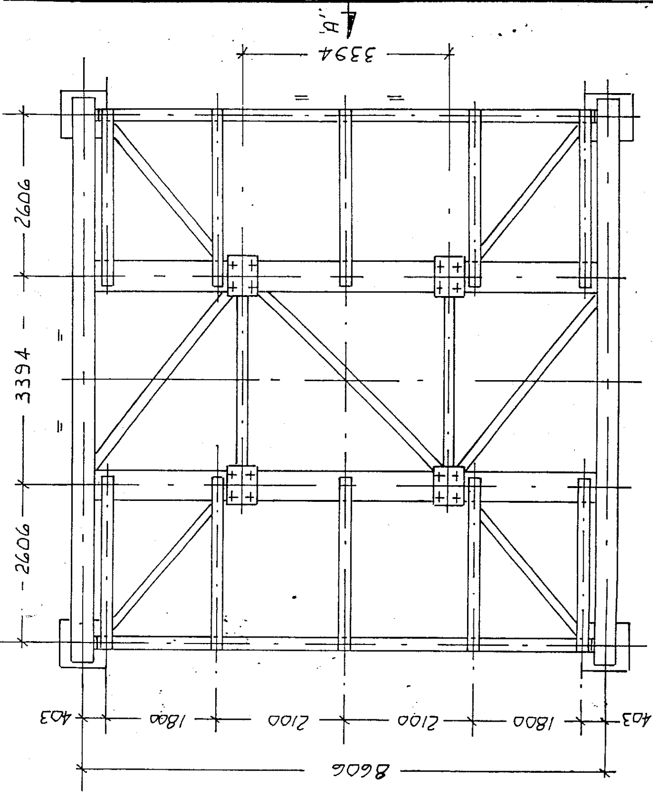
G.A. PLAN OF RAIL GRILLAGE 1:50
