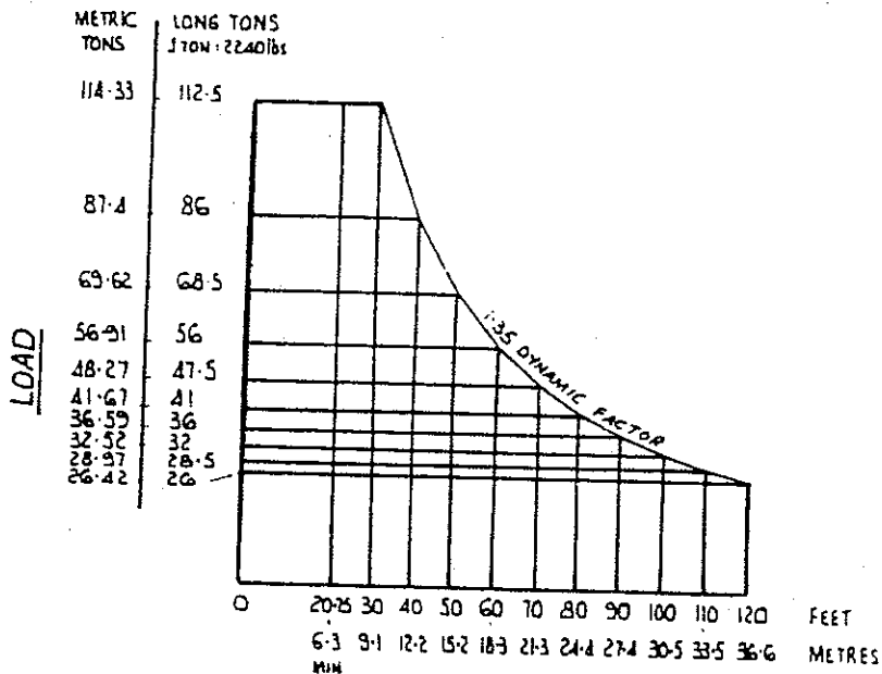
RADIUS LOAD CAPACITY CHART 120'-0" LONG JIB - 5 FALL HOOK
