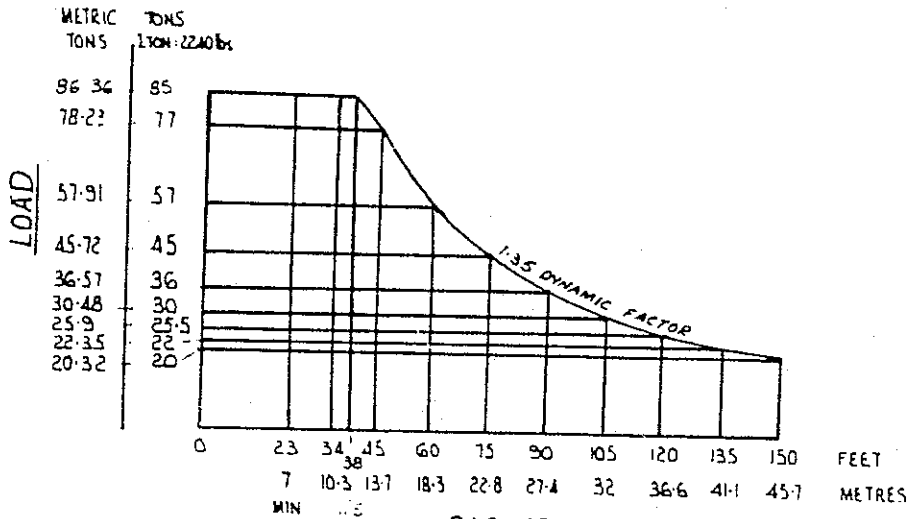
RADIUS LOAD CAPACITY CHART 150'-0" LONG JIB - 4 FALL HOOK
